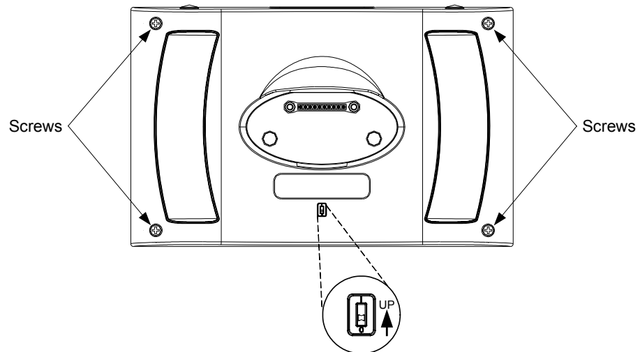
Bottom View Showing Battery Switch and Screw Locations
